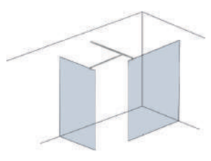
Corner Two glass panels installed with two support arms and a T piece
